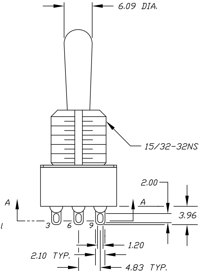
CONTACT CONFIGURATION
