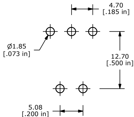
P.C. MOUNTING
