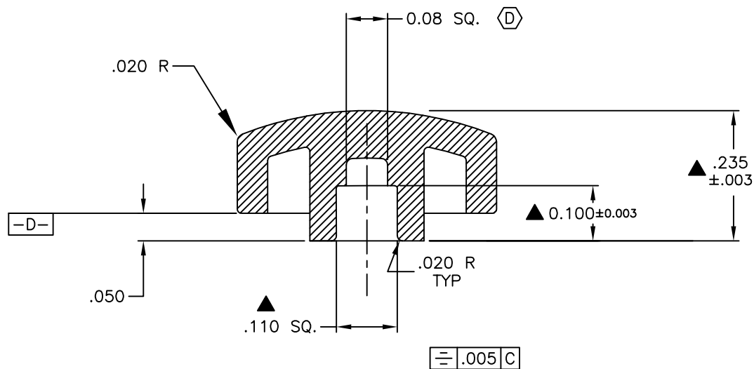
CROSS SECTION SCALE 4:1
