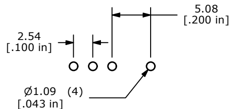
P.C. MOUNTING
