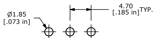
P.C. MOUNTING
