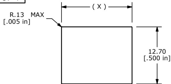
PANEL MOUNTING
