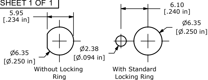
PANEL MOUNTING
