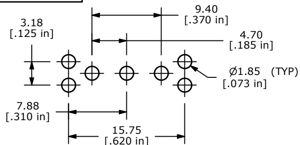
P.C. MOUNTING
