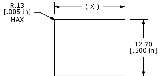
PANEL MOUNTING
