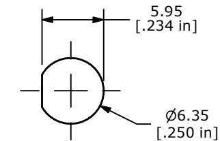
PANEL MOUNTING
