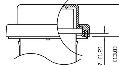
ASSEMBLED VIEW
