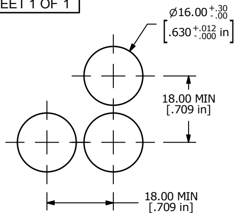
PANEL MOUNTING
