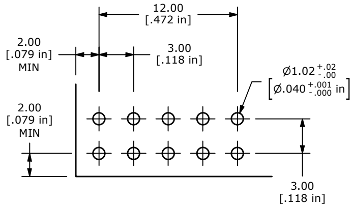
PCB LAYOUT
