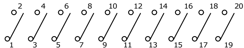
▲ CIRCUIT - 10 POSITION
