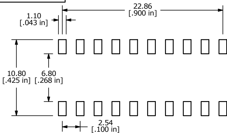
P.C.B. MOUNTING
