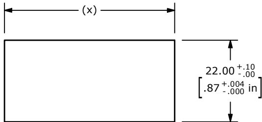
PANEL CUTOUT
