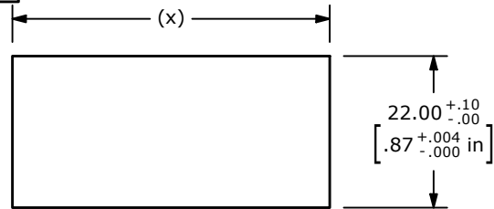
PANEL CUTOUT
