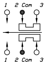
CIRCUIT: DPDT CONTACT CONFIGURATION
