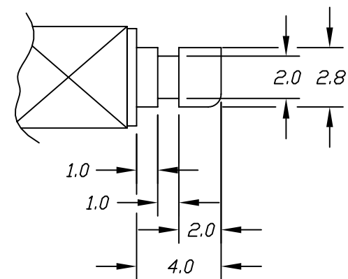
(ACTUATOR DETAIL) SCALE 4:1
