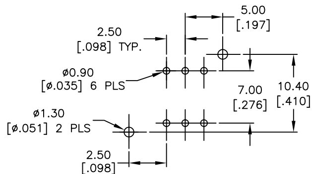
RECOMMEND P.C.B. HOLES
