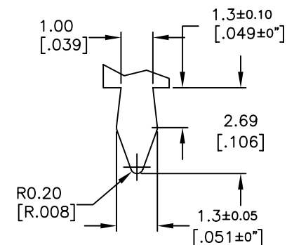
DETAIL-A- (6:1)
