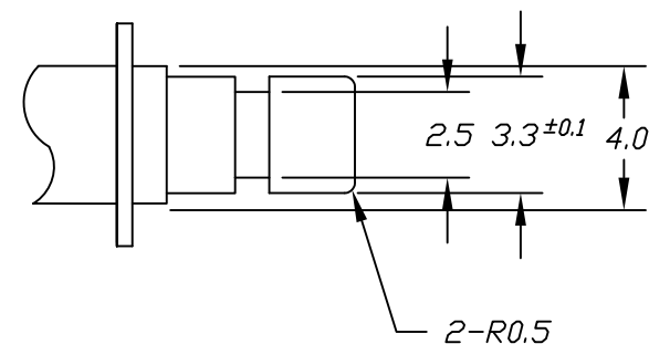
CONTACT CONFIGURATION
