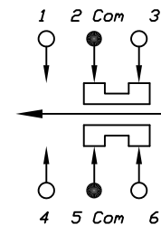
CIRCUIT: DPDT
