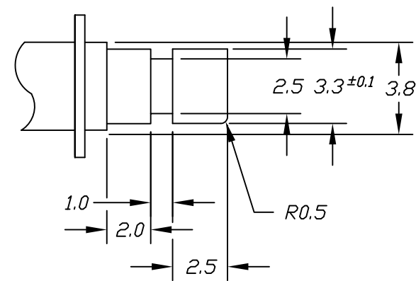
(ACTUATOR DETAIL) SCALE 4:1
