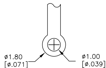
DETAIL-A- (SCALE 6:1)
