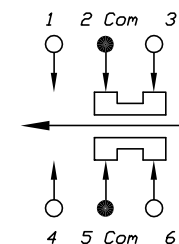
CIRCUIT: DPDT
