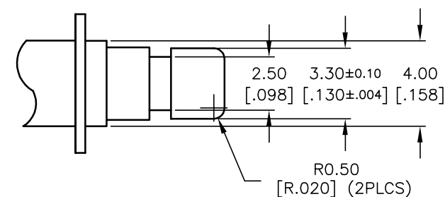
CONTACT CONFIGURATION
