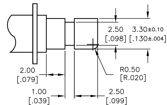
(ACTUATOR DETAIL) SCALE 4:1
