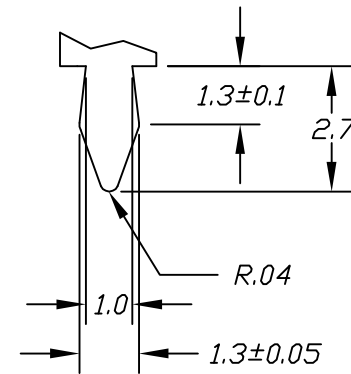
DETAIL-A- (6:1)
