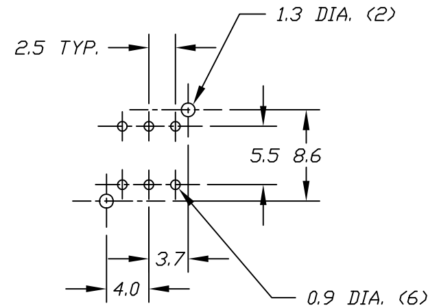
RECOMMEND P.C.B. HOLES
