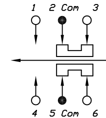
CIRCUIT: DPDT
