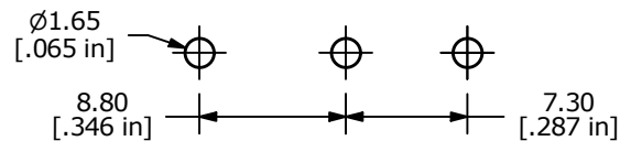
P.C. MOUNTING
