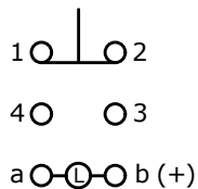
SPDT CONTACT CONFIGURATION
