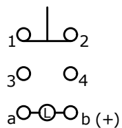
SPDT CONTACT CONFIGURATION (MOMENTARY)
