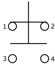
SCHEMATIC DPST Non-Illuminated ON (OFF)/OFF (ON) ( ) = MOMENTARY
