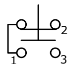
▲ CONTACT CONFIGURATION SPDT ON - (ON) ( ) = MOMENTARY
