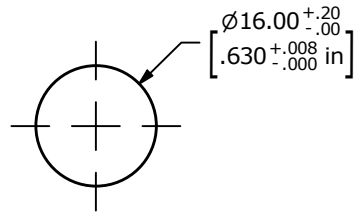
PANEL CUTOUT MAX. PANEL THICKNESS 14mm
