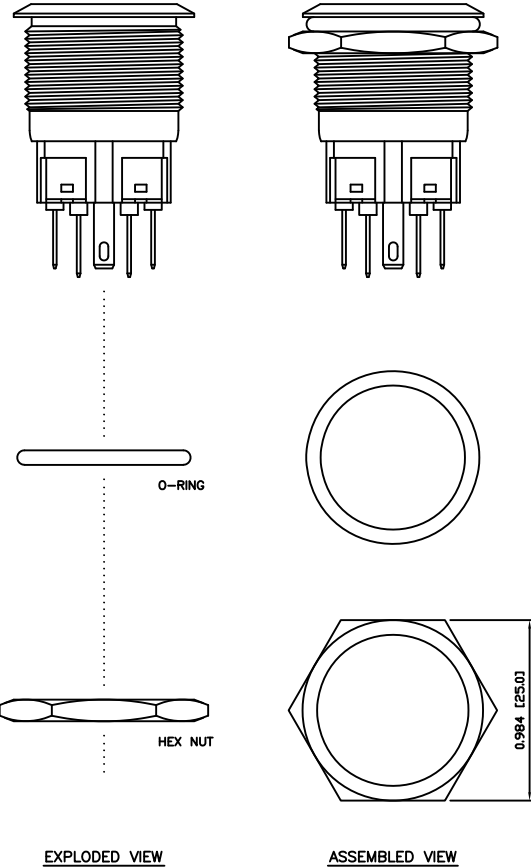
EXPLODED VIEW
