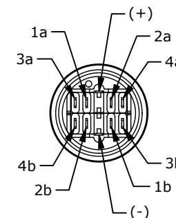
BOTTOM VIEW SHOWN WITHOUT WIRING
