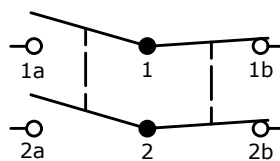
CIRCUIT: DPDT
