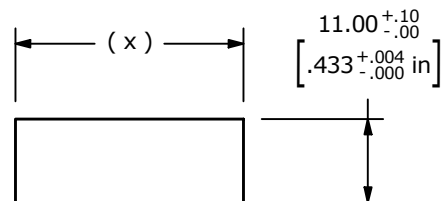
PANEL CUTOUT
