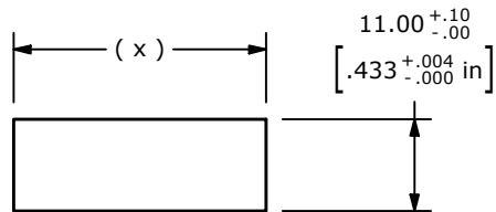
PANEL CUTOUT
