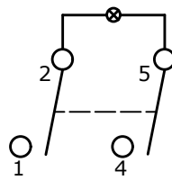
CIRCUIT: DPST OFF - ON
