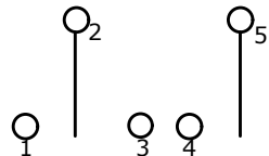
▲ CIRCUIT: DPDT ON - OFF - ON MAINTAINED
