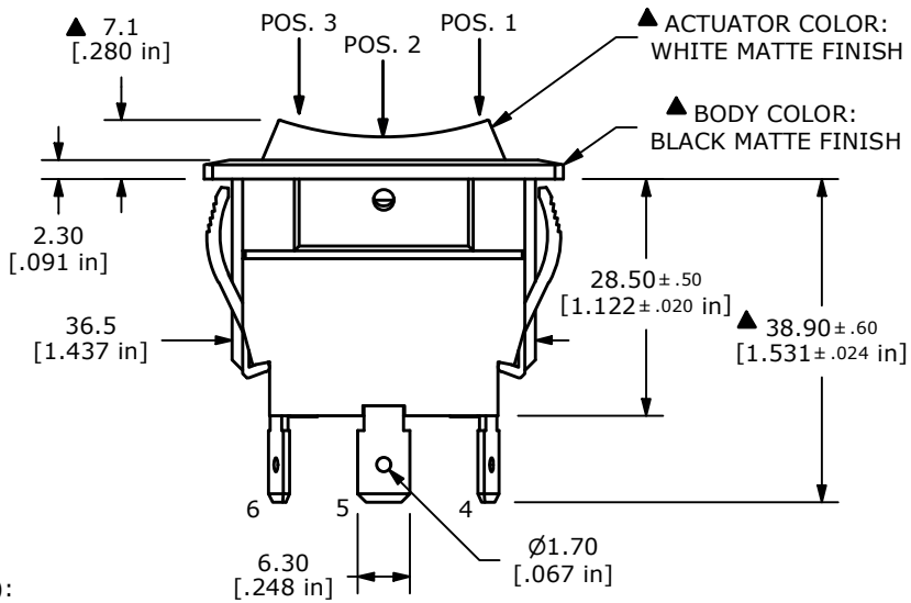
▲ CIRCUIT: DPDT ON - OFF - ON MAINTAINED
