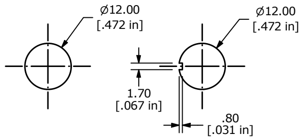
RECOMMENDED PANEL CUT-OUTS
