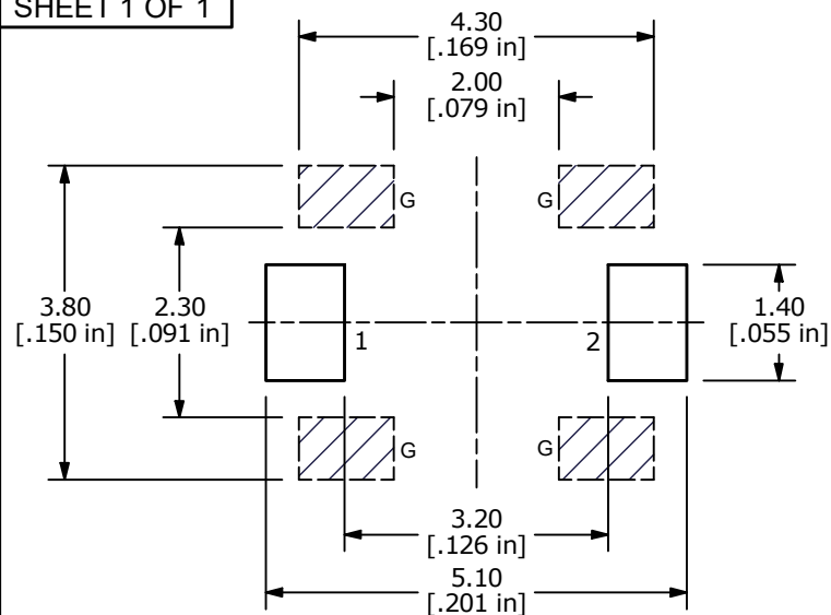
P.C.B LAYOUT (GROUND TERMINALS OPTIONAL)
