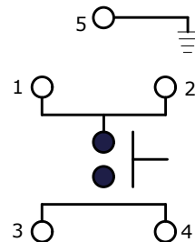
▲ CIRCUIT: SPST
