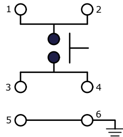
CIRCUIT: SPST
