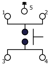
▲ CIRCUIT: SPST
