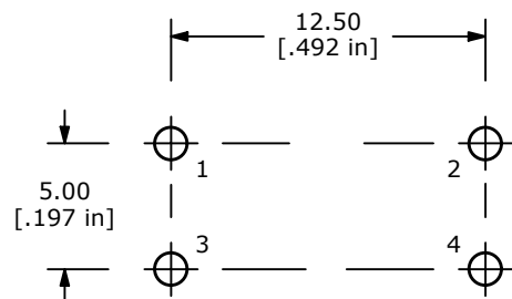
PCB MOUNTING
