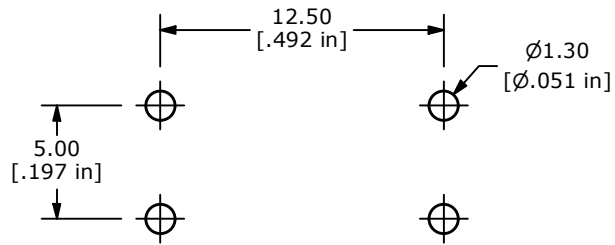
P.C.B. MOUNTING
