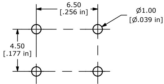
P.C. MOUNTING
