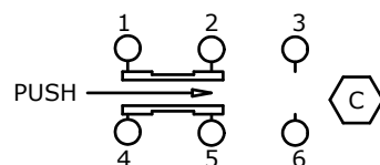
CIRCUIT DIAGRAM (DPDT) MAKE BEFORE BREAK ▲
