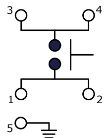
CIRCUIT: SPST ▲
