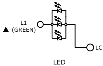
CIRCUIT LAYOUT
