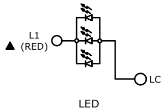
▲ CIRCUIT LAYOUT
