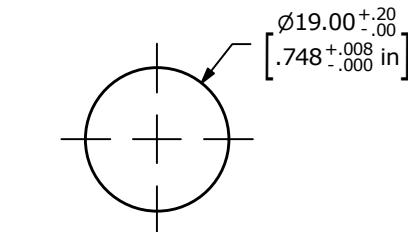
PANEL CUT-OUT PANEL THICKNESS 1-10mm
