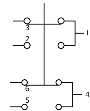
LED 1 (+) LED 2 (-) SCHEMATIC ON - ON DPDT Illuminated
