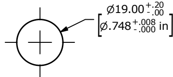
RECOMMENDED PANEL CUTOUT MAX. PANEL THICKNESS 10.0 [.39 in]
