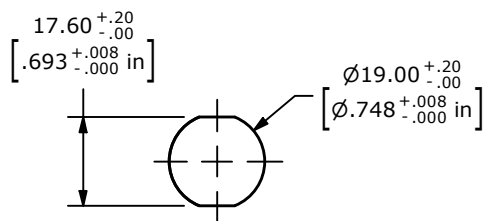
RECOMMENDED PANEL CUTOUT MAX. PANEL THICKNESS 10mm
