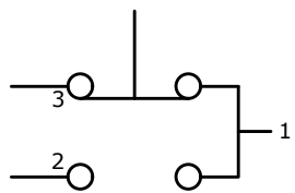
SCHEMATIC ▲ ON - (ON) SPDT NON-ILLUMINATED (ON) = MOMENTARY FUNCTION
